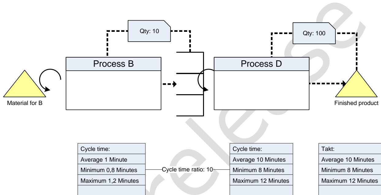
Figure 14: Activity cycle time example
